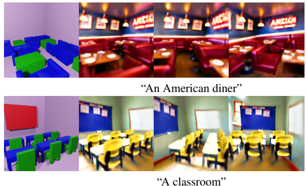
Figure 5: Scene generation results. Our method is able to handle complex scenes with multiple repeating objects.
