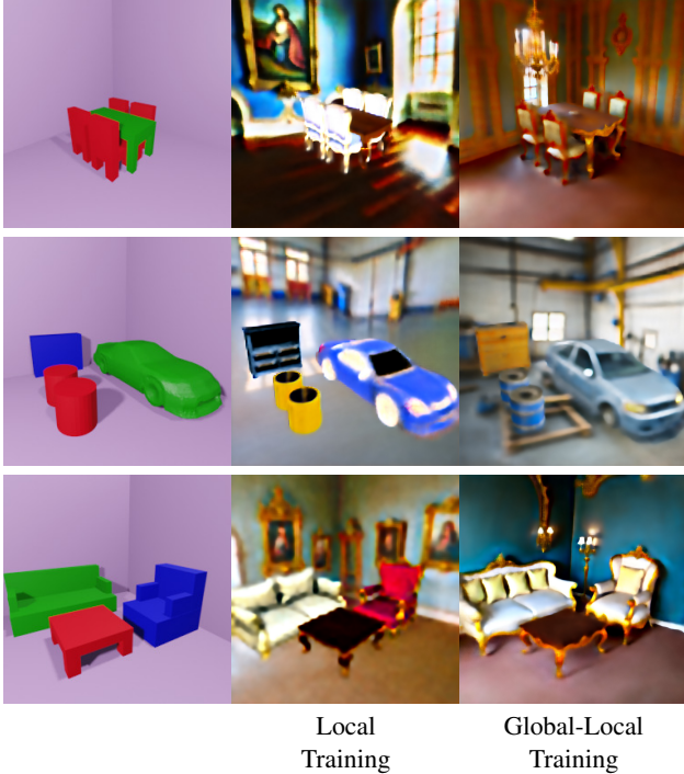
Figure 9: Impact of Global-Local training. Here we show the importance of global training for three different scenes. Observe how our Global-Local training policy results in more coherent scenes, compared to scenes where each object is optimized independently that are inconsistent.
