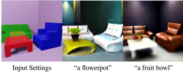
Figure 6: Objects with no shape priors. For some objects it is beneficial to define only their location without explicitly stating their shape. Here we highlight how different objects can be generated on top of the table.
